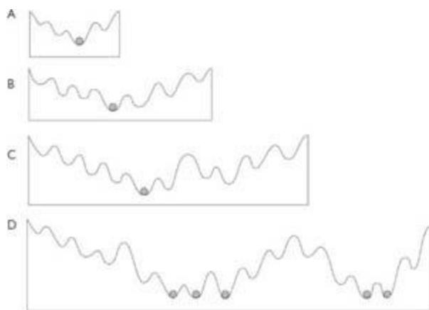
Figure 8. A diagrammatic representation of the possible structures of systems of increasing complexity. In A there is a unique minimum-energy structure, but in D several different possible structures are equally stable.
